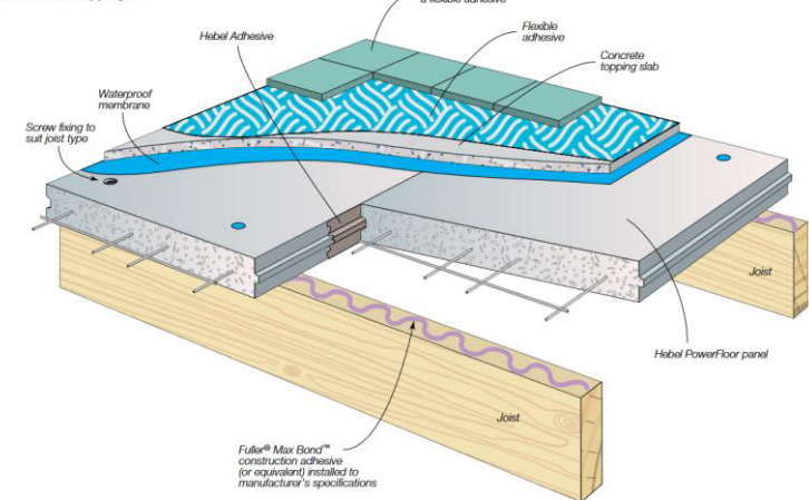
Figure 3.2.5 Hebel PowerFloor system with 8mm ceramic tiles on 50mm topping slab
